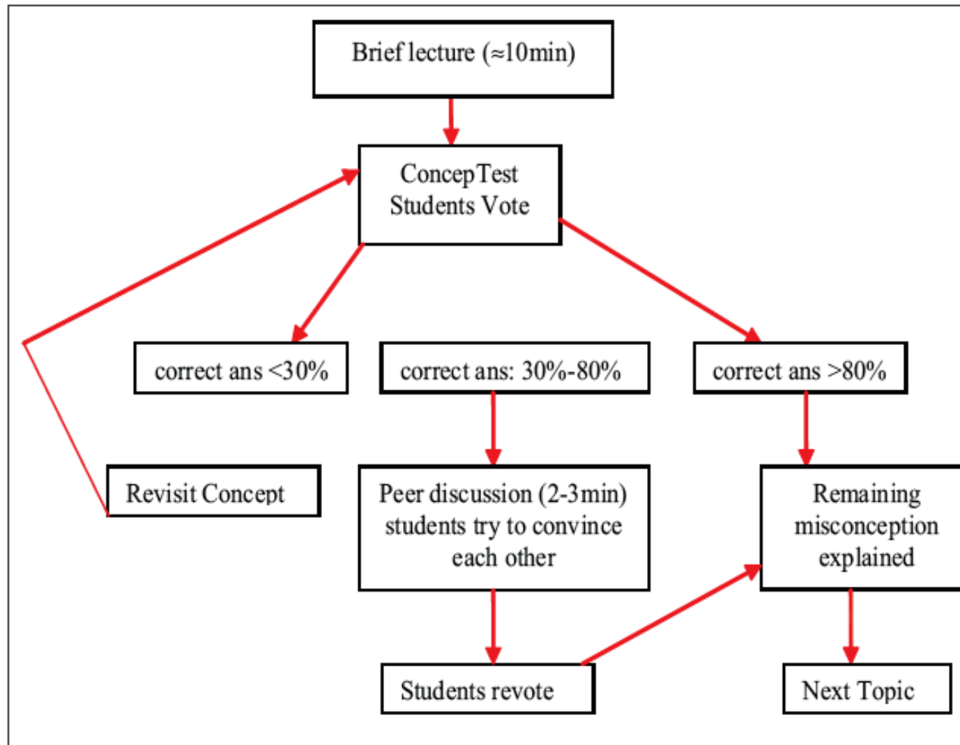
1: Fig. 1. A Peer Instruction Implementation Algorithm.
